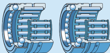
NX series
