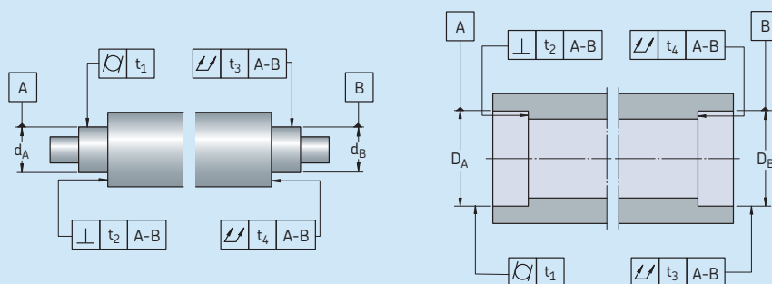
Accuracy of form and position for bearing seats on shafts and in housings
