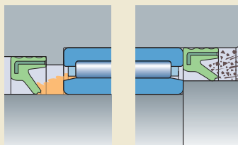
Primary lip facing inward
