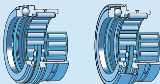
NKX series
