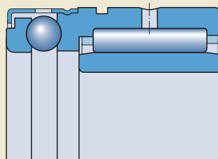
NX series
