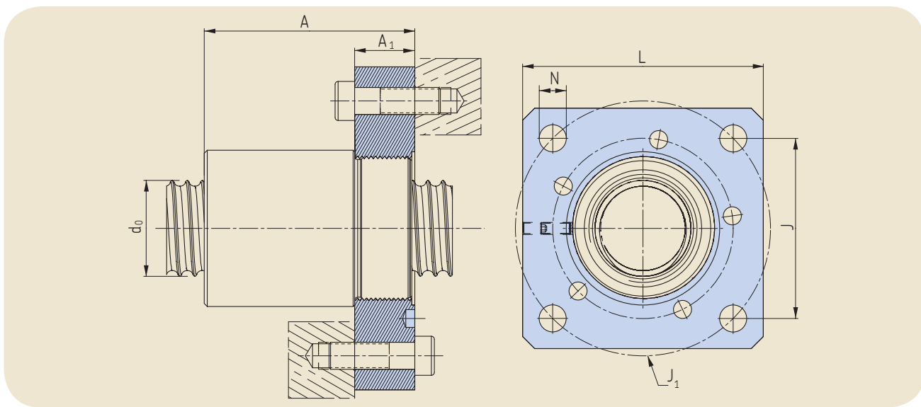
SX nut with flange
