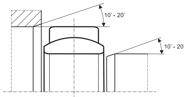
Figure 2: Centering chamfers
