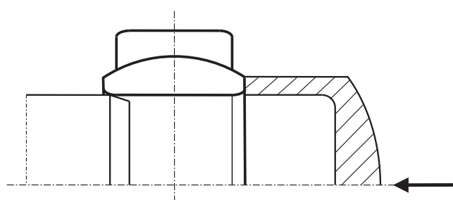
Figure 3: Installation tool
