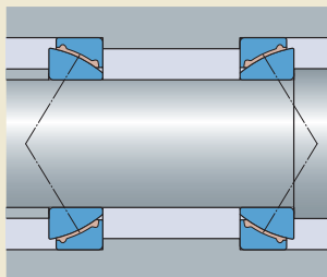
Angular contact spherical plain bearings, back-to-back arrangement
