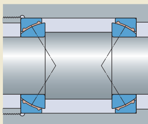
Angular contact spherical plain bearings, face-to-face arrangement
